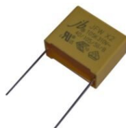
PI05X310VAC CAPACITOR POL MET 1UF 310VAC X2 22.5MM
