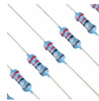
RE361F RESISTENCIA METALFILM 0.4W 1% 360 OHM
