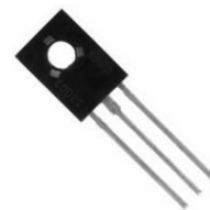
BD140 TRANSISTOR BIPOLAR PNP 1.5A 80V
